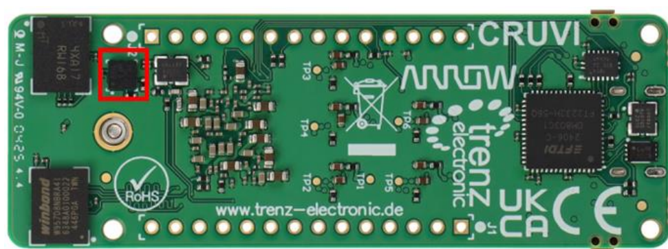
Figure 3-4 : Accelerometer location
